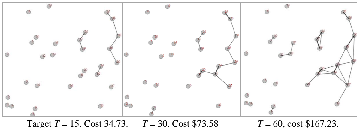
Target T = 15 . Cost 34.73. T = 30 . Cost 73.58 T = 60 , cost 167.23. Figure 3. With an increasing budget, connectivity may increase within existing connected areas. Edge thickness indicates degree of connectivity.
